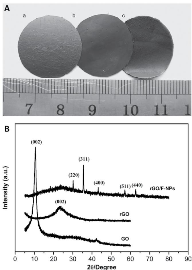
Fig. 2 - (A) Photographs of graphene oxide (GO) (a), reduced graphene oxide (rGO) (b) and rGO/ Fe 3 O 4 nanoparticle (F-NP) (c) (200 mg) films; (B) their corresponding X-ray diffraction (XRD) patterns.
