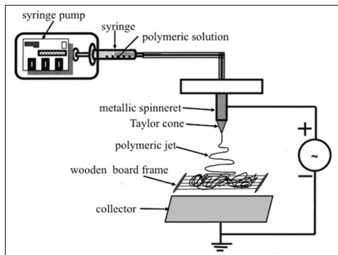
Fig. 1 - Home-made electrospinning apparatus for the fabrication of the nano/micro hybrid scaffold.
