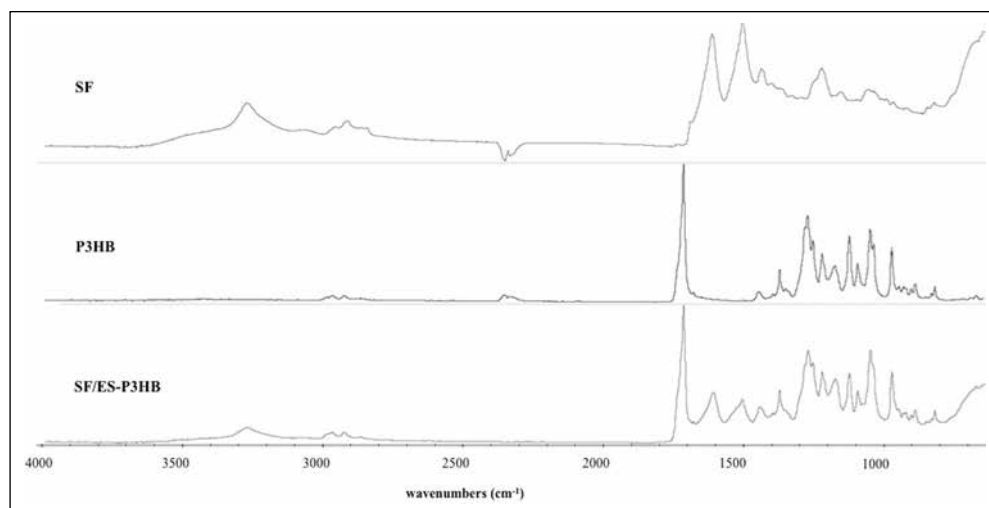
Fig. 7 - Attenuated total reflectance–Fourier transform infrared (ATR-FTIR) spectra of SF, P3HB nanofibers and SF/ES-P3HB. ES = electrospun; P3HB = poly(3-hydroxybutyrate); SF = silk fibroin.
