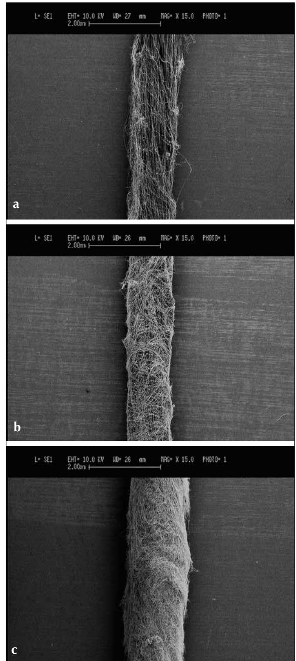
Fig. 3 - The effect of the electrospinning coating time on nano/micro hybrid scaffolds of silk/ES-P3HB in 5 minutes (a), 15 minutes (b) and 25 minutes (c). Scale bar: 2 mm. ES = electrospun; P3HB = poly(3-hydroxybutyrate).
